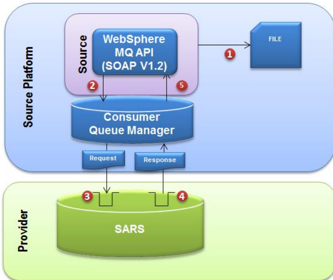
Figure 7: Typical interaction between an Application and SARS using the MQ FTE protocol:
